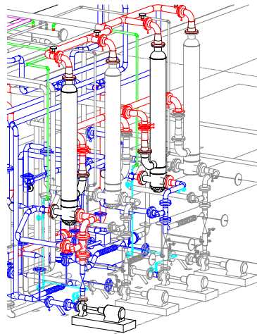
3-D design of a hot oil system.
